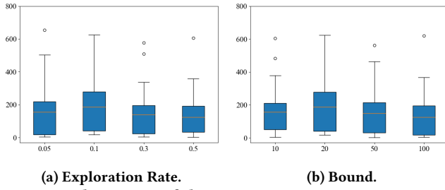
(a) Exploration Rate. (b) Bound. Figure 4: The impact of the parameter settings on SJFuzz in all benchmarks.
