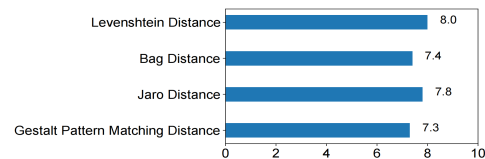
Figure 7: Average unique discrepancies exposed by different distance metrics in all benchmarks.
