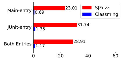
Figure 5: Average seed-mutant Levenshtein Distance.
